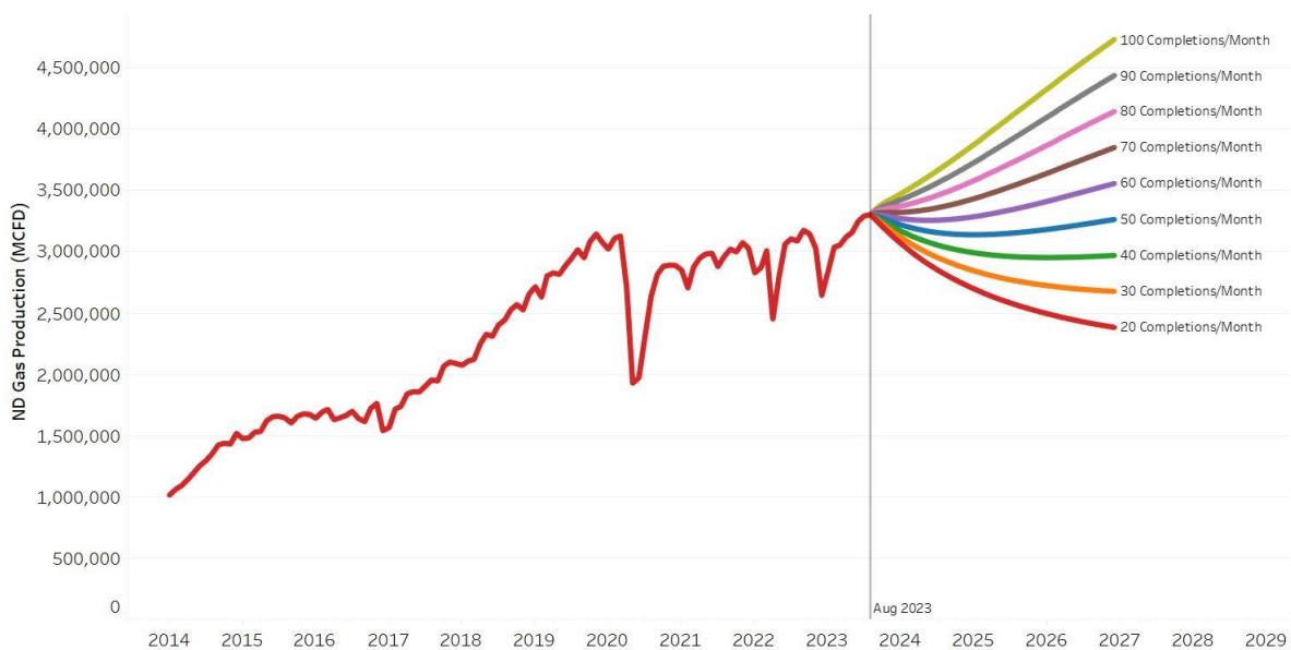
Figure 5. North Dakota natural gas production under various completion scenarios
