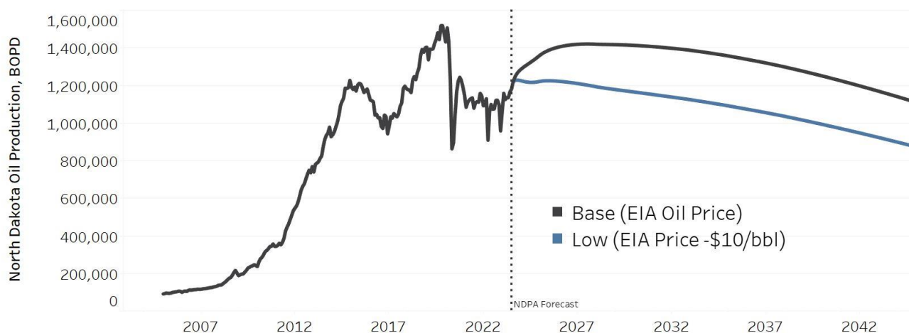
Figure 2. Long term crude oil production forecast for North Dakota starting in Aug. 2023
