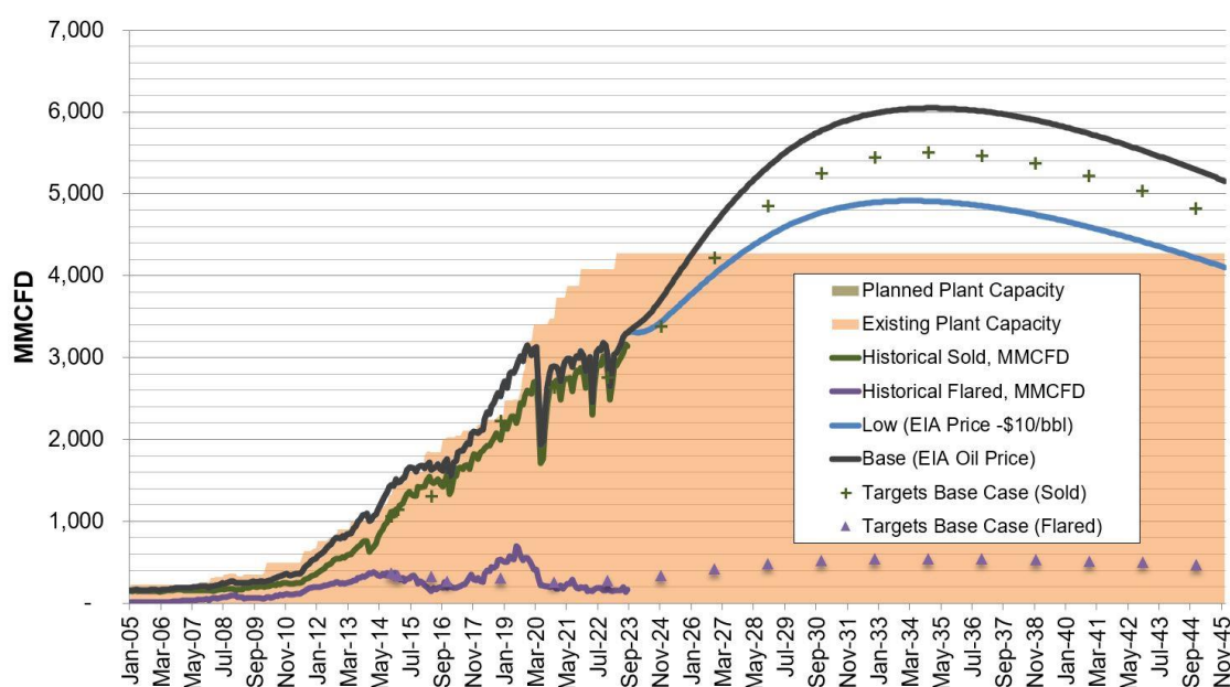
Figure 7. North Dakota natural gas processing plant intake capacity, gas production, gas forecast, and NDIC capture targets. (Forecast starts in Aug. 2023)
