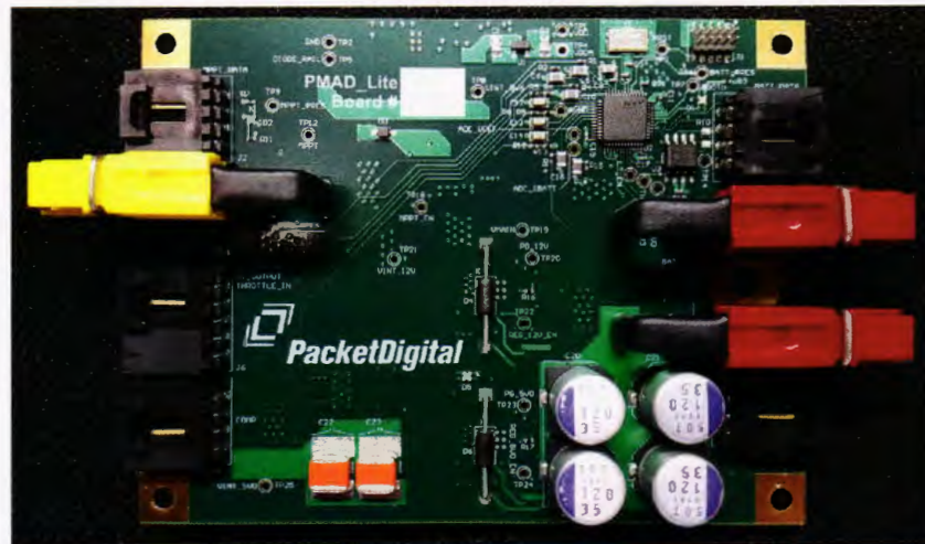
Figure 9: PMAD Lite
