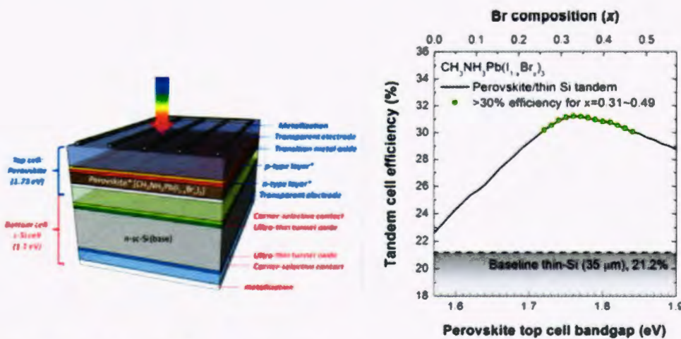
Figure 5: The left hand figure show the schematic diagram of the NRL developed Perovskite/Si tandem solar cell and on the right are NRL modeled results showing the potential of achieving >30% efficiency.
