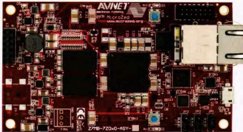
Figure 21: Xilinx Zynq Eval Board
