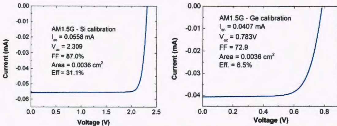
Figure 4: The MJ stacked solar cells under development at NRL have achieved a total of 37.6 % efficiency by stacking two MJ solar cells into a single device. This is a four terminal device, so the top and bottom junctions are measured independently.
