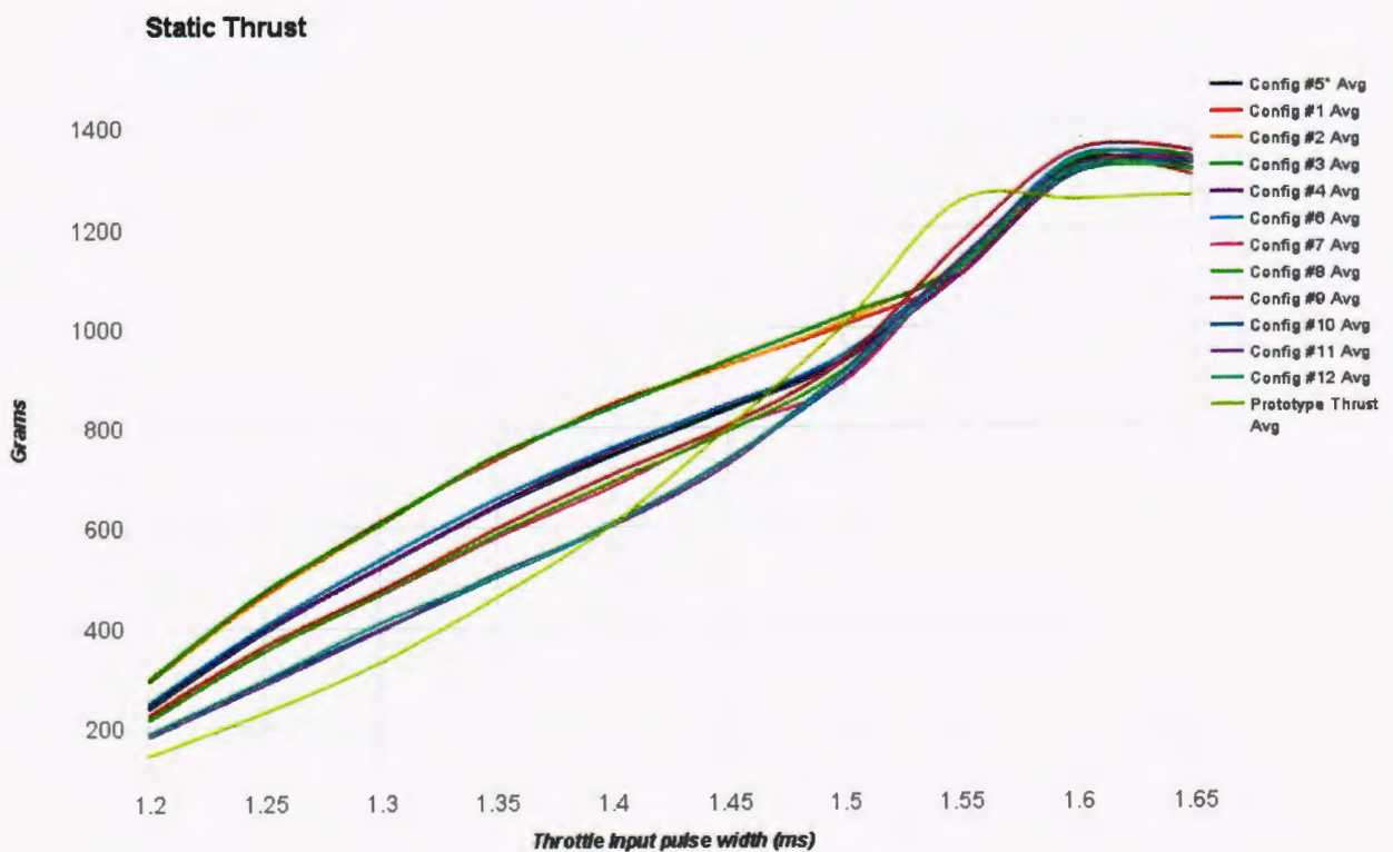
Figure 18: Static Thrust by ESC Configuration
