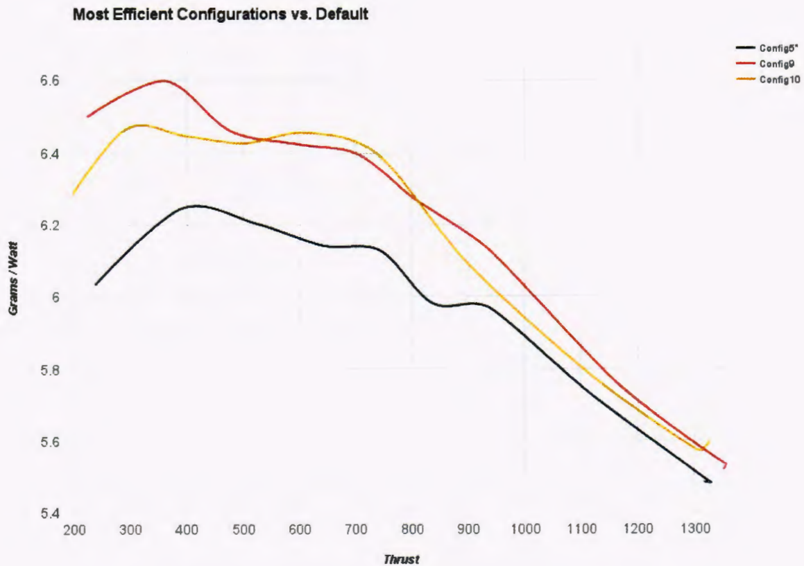
Figure 20: Thrust Efficiency by ESC Config, Most Efficient
