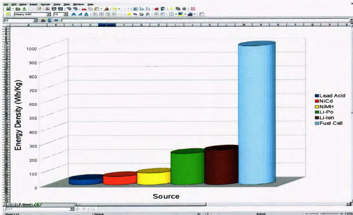
Figure 13: Fuel cell energy density comparison
