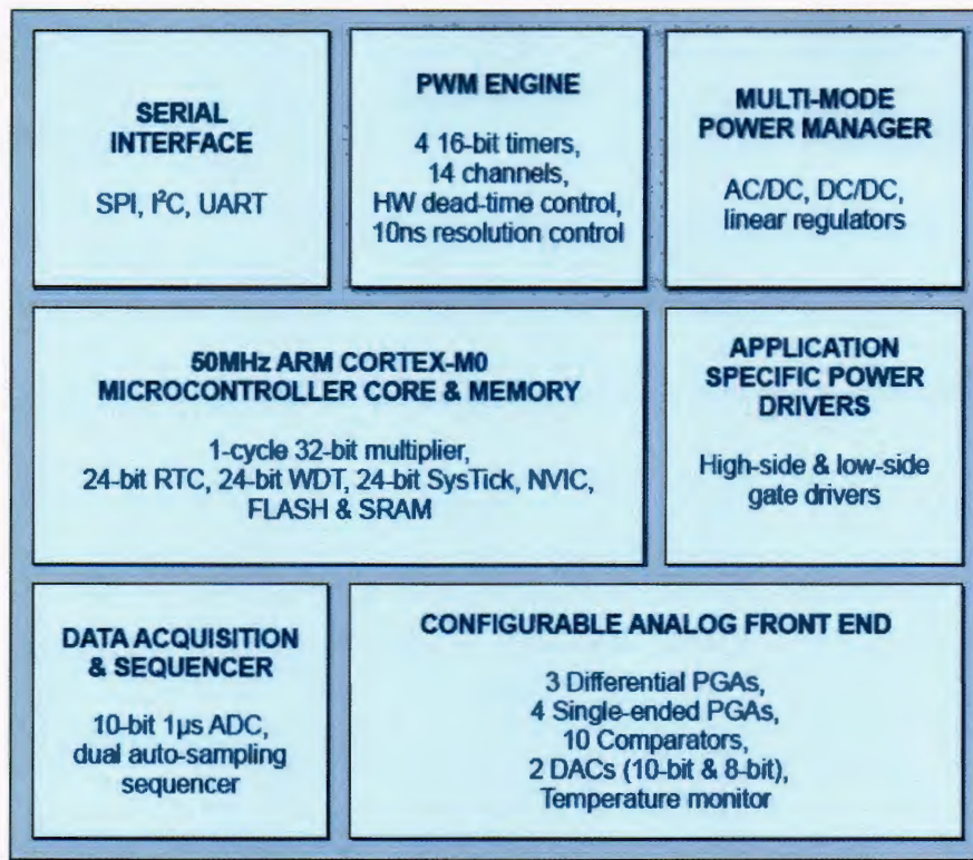
Figure 16: Power Application Controller
