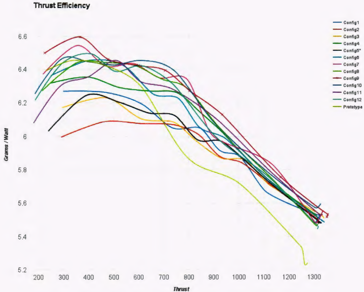
Figure 19: Thrust Efficiency by ESC Configuration
