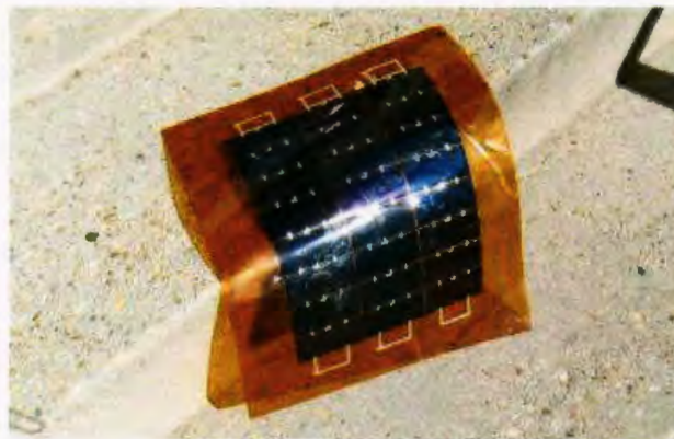
Figure 3: Flexible solar array material being used to develop the UAS wing skin. This example uses multijunction, large-area solar cells with flexible encapsulation.
